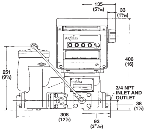
1" 4D-MD with 800 Series Register
