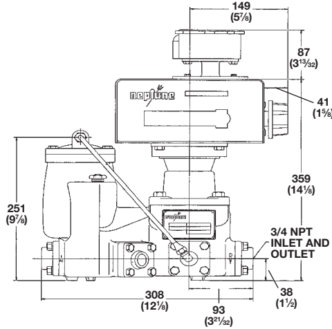
1" 4D-MD with 600 Series Register
