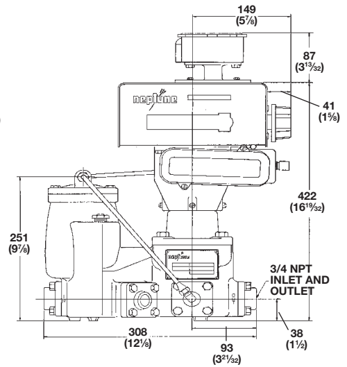
1" 4D-MD with 600 Series Register and ATC
